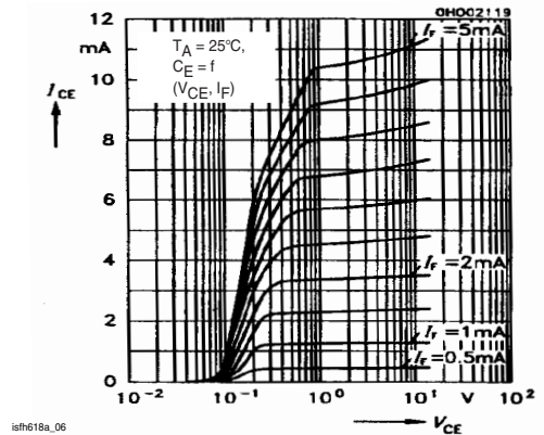
Figure 9. Output Characteristics
