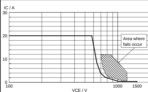
Fig.13. Reverse bias safe operating area. T_j \leq T_{j\text{max}}
