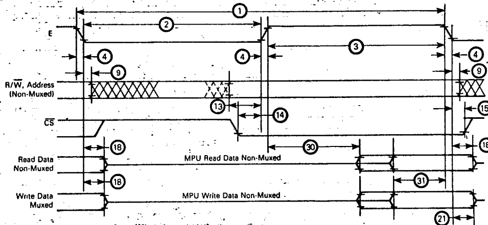
FIGURE 3 - BUS TIMING
