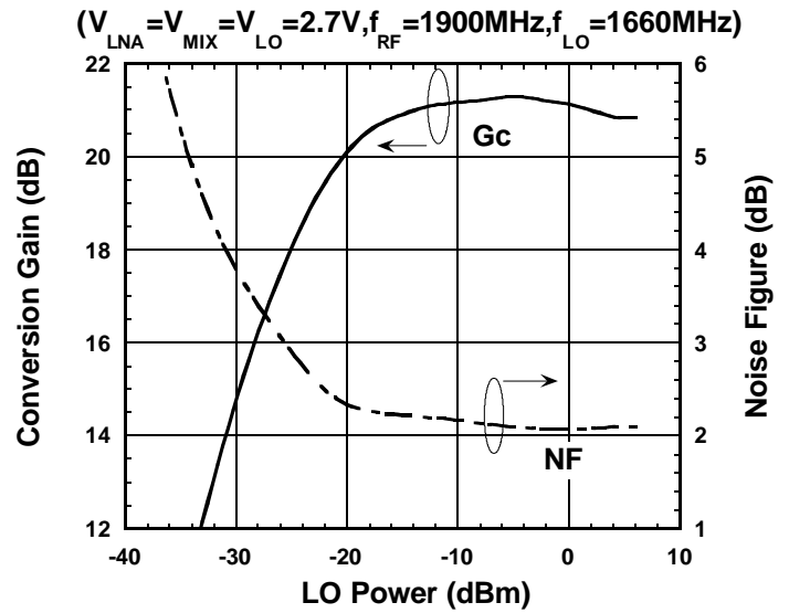
Conversion Gain , Noise Figure vs. LO Power ( V_{LNA}=V_{MIX}=V_{LO}=2.7\text{V}, f_{RF}=1900\text{MHz}, f_{LO}=1660\text{MHz} )
