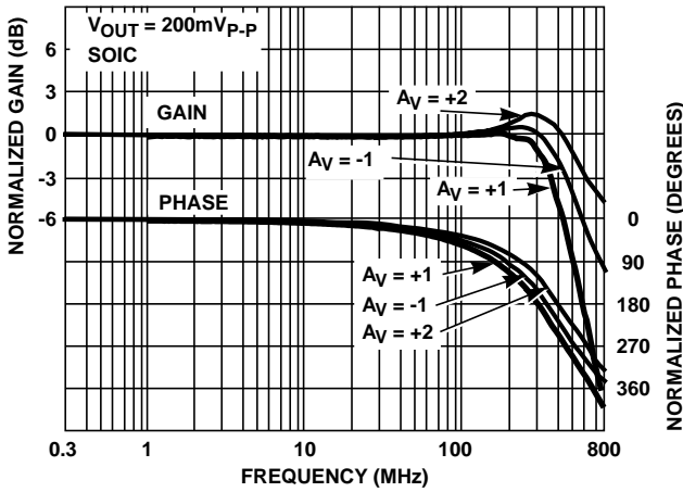
FIGURE 12. FREQUENCY RESPONSE
