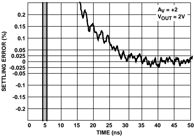
FIGURE 20. SETTling RESPONSE
