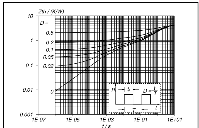
Fig.4. Transient thermal impedance. Z_{th-jhs} = f(t) ; parameter D = t_p / T
