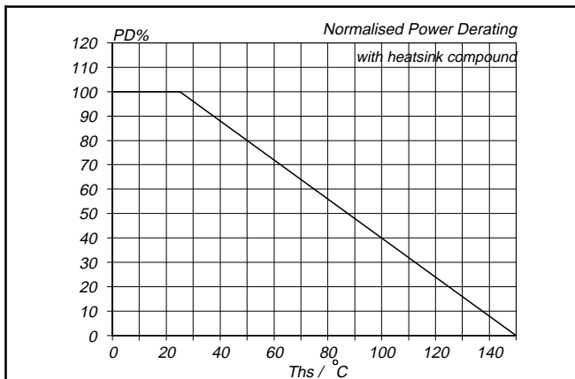
Fig.1. Normalised power dissipation. PD\% = 100 \cdot P_D / P_{D\ 25\text{ }^{\circ}\text{C}} = f(T_{hs})
