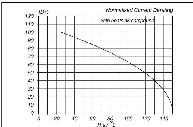
Fig.2. Normalised continuous drain current. ID\% = 100 \cdot I_D / I_{D\ 25\text{ }^{\circ}\text{C}} = f(T_{hs}) ; conditions: V_{GS} \geq 10\text{ V}
