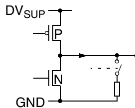
Fig. 5-12: Digital Output Pins MCLK, RD, STRB, DAO
