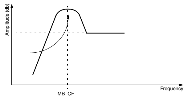
Fig. 3–5: Adding harmonics
