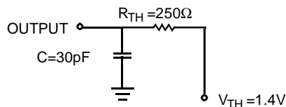
(b) Thévenin Equivalent (Load 2)
