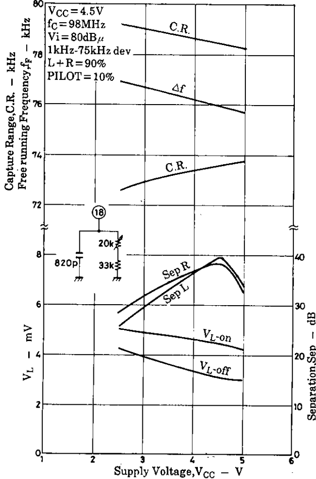
MPX V_{CC} Characteristics(2)
