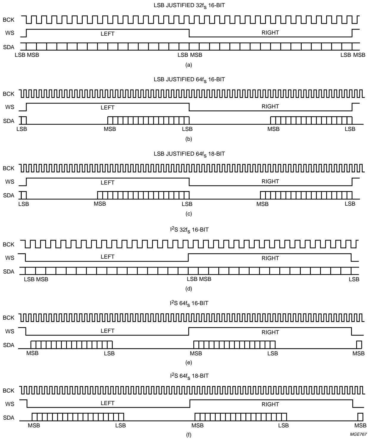
Fig.3 DAC and ADC data formats (continued in Fig.4).
