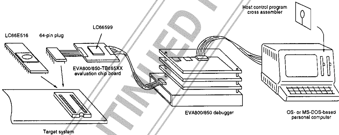
Figure 10. Development tools
