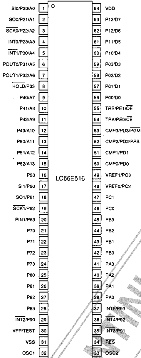
Figure 11. LC66E516 pinout
