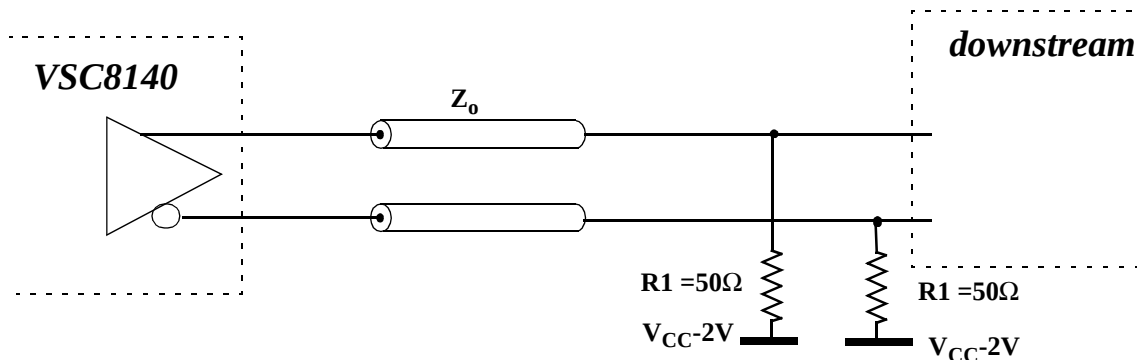
Figure 4: DC Termination of Low-Speed LVPECL RXCLK16O, RXCLK16_32O, TXCLK16O Outputs
