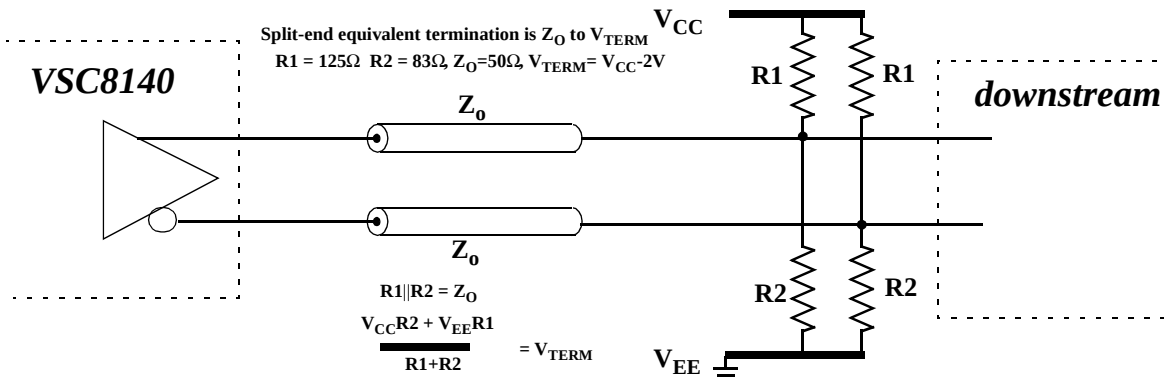
Figure 4: DC Termination of Low-Speed LVPECL RXCLK16O, RXCLK16_32O, TXCLK16O Outputs
