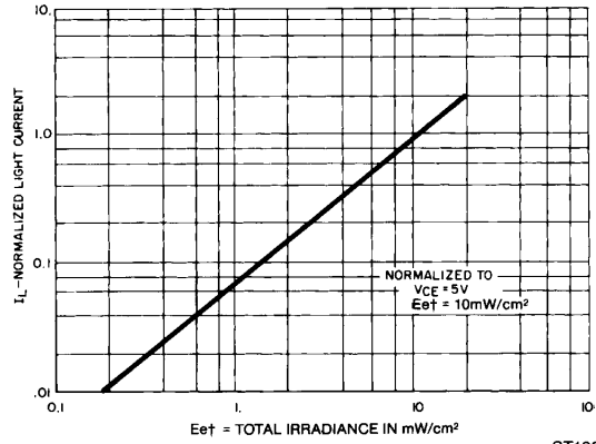
Fig. 2. Normalized Light Current vs. Radiation ST1087
