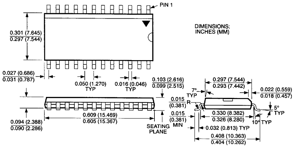
24-Pin Wide SOIC (WM)
