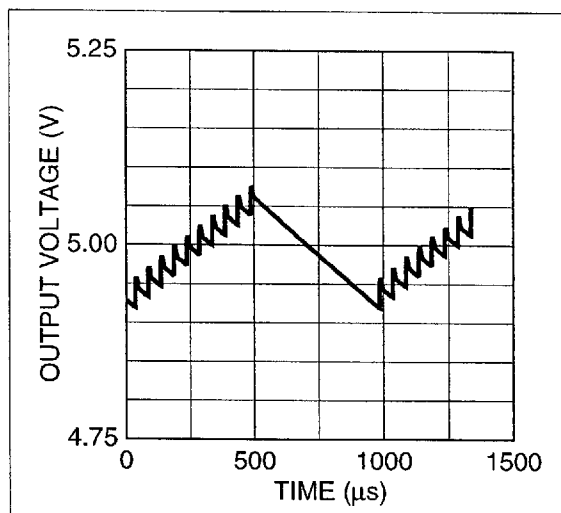
Figure 4. Output Ripple
