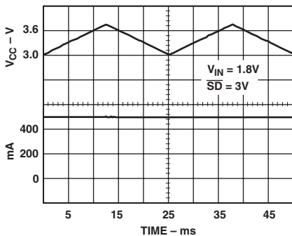
TPC 25. Current Limiting from V_C
