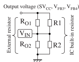
Figure 4. Resistor connecting diagram to set output voltage
