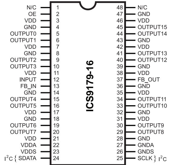
48-Pin SSOP
