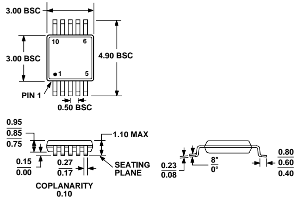
COMPLIANT TO JEDEC STANDARDS MO-187BA Figure 44. 10-Lead Mini Small Outline Package [MSOP] (RM-10) Dimensions shown in millimeters
