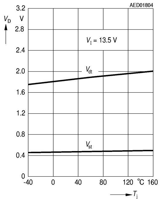
Switching Voltage V_{dt} and V_{st} versus Temperature T_j
