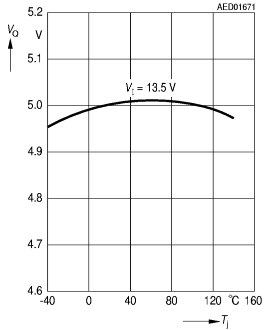
Output Voltage V_O versus Temperature T_j
