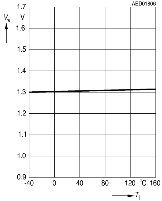
Reset Switching Threshold V_{re} versus Temperature T_j
