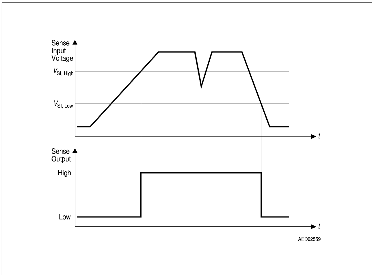
Sence Timing Diagram
