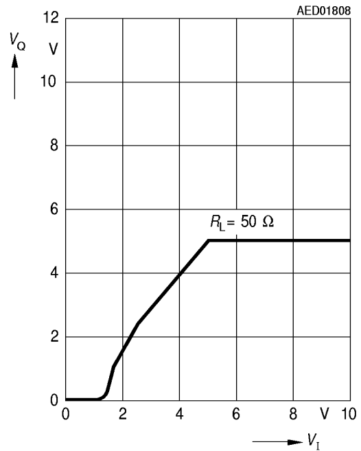
Output Voltage V_O versus Input Voltage V_I
