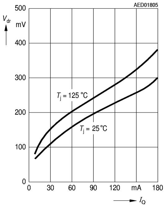
Drop Voltage V_{dr} versus Output Current I_O
