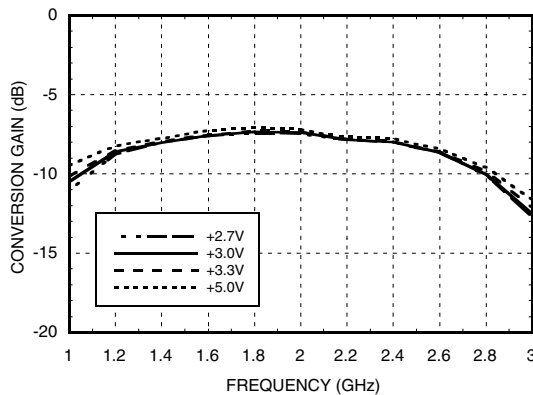
Conversion Gain vs. Vdd @ LO = 0 dBm
