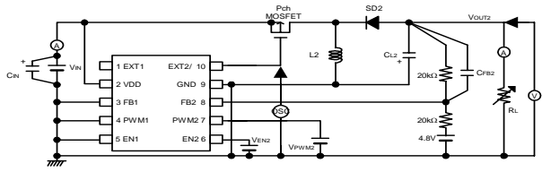
Circuit 7
