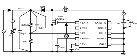
Circuit 5
