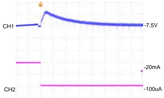
200usec/div CH1:Vout2 , AC-COUPLED, 50mV/div CH2:Iout2 , 10mA/div
