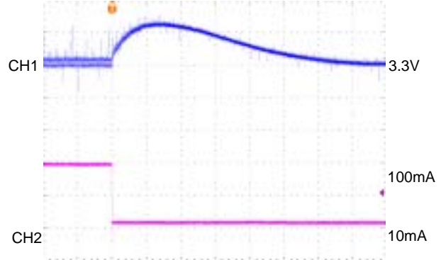
200usec/div CH1:V OUT1 , AC-COUPLED, 50mV/div CH2:I OUT1 , 50mA/div
