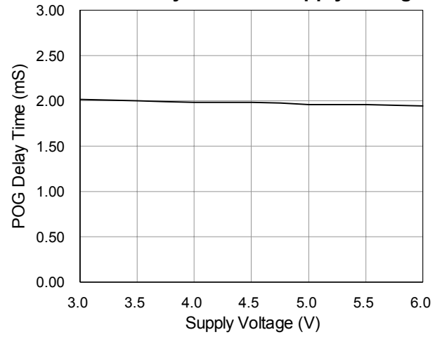
POG Delay Time vs. Supply Voltage
