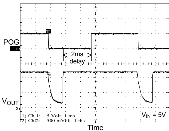
POG Response vs. VOUT
