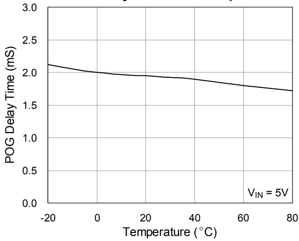
POG Delay Time vs. Temperature
