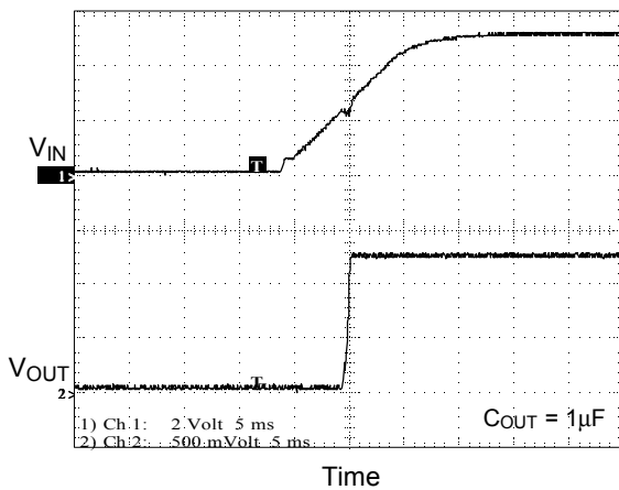
Under Voltage Lock Out
