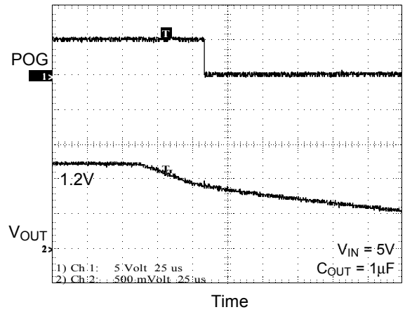
POG Response at Power Down
