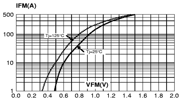
Fig. 7: Forward voltage drop versus forward current (maximum values, per diode).
