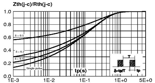
Fig. 4: Relative variation of thermal impedance junction to case versus pulse duration (per diode).
