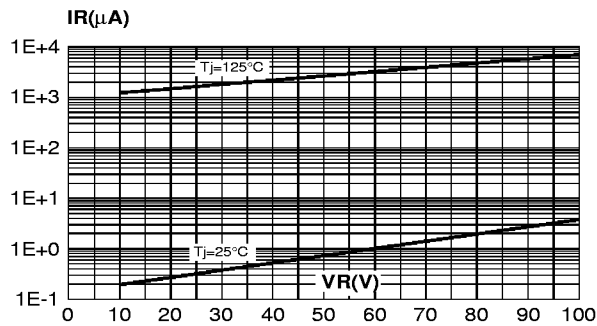
Fig. 5: Reverse leakage current versus reverse voltage applied (typical values, per diode).
