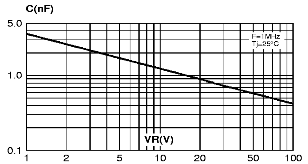
Fig. 6: Junction capacitance versus reverse voltage applied (typical values, per diode).
