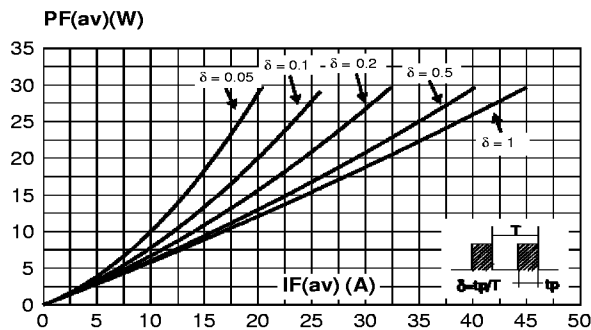
Fig. 1: Average forward power dissipation versus average forward current (per diode).
