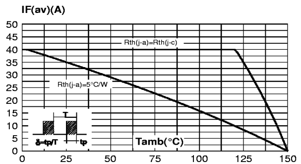
Fig. 2: Average forward current versus ambient temperature ( \delta=0.5 , per diode).
