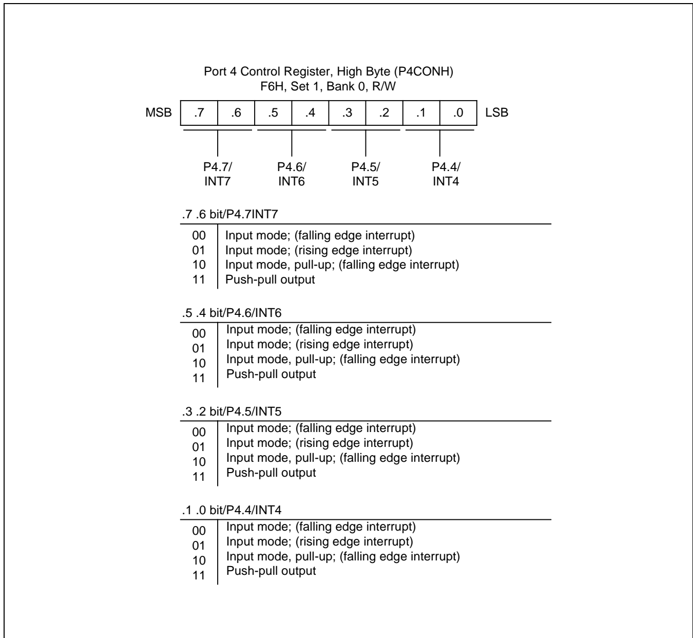
Figure 9-7. Port 4 High-Byte Control Register (P4CONH)
