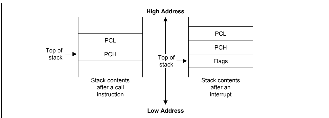
Figure 2-15. Stack Operations
