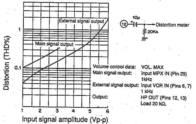
Distortion characteristics
