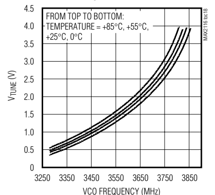
VCO_4: V TUNE vs. VCO FREQUENCY
