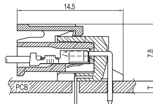
PCB ASSY
