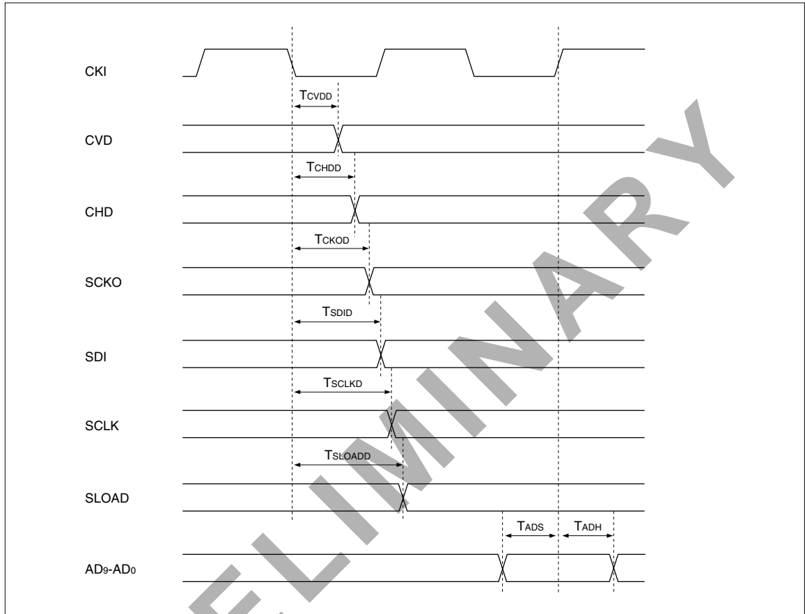
Fig. 3 CMOS Image Sensor Interface Timing
