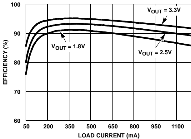
FIGURE 1. EFFICIENCY vs LOAD CURRENT ( V_{IN} = 5.0V )
