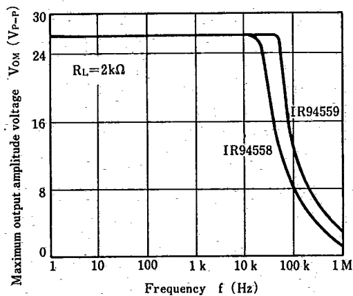
Maximum output amplitude voltage—Frequency Characteristics
