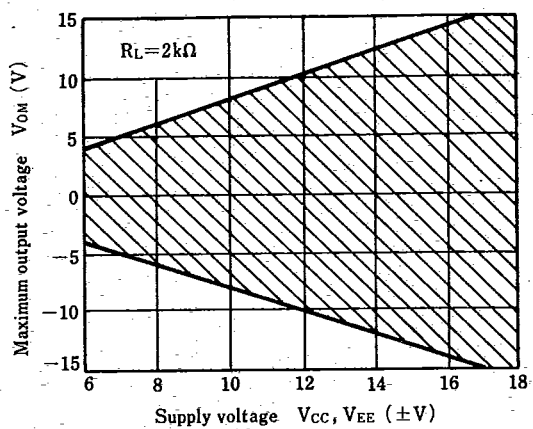
Maximum output voltage—Supply voltage Characteristics
