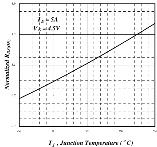
Fig 4. Normalized On-Resistance
