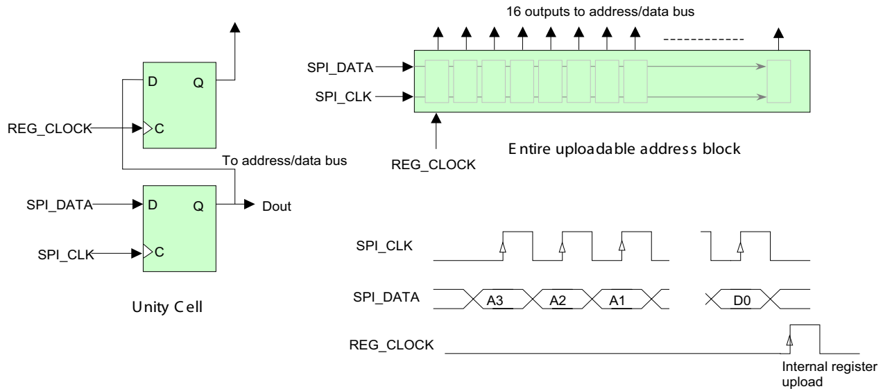
Figure 18. SPI Interface
