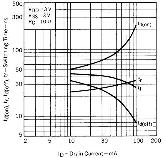
SWITCHING CHARACTERISTICS
