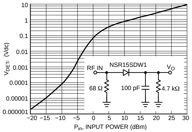
Figure 8. Typical Output Voltage versus Input Power, Large Signal Detector Operating at 915 MHz
