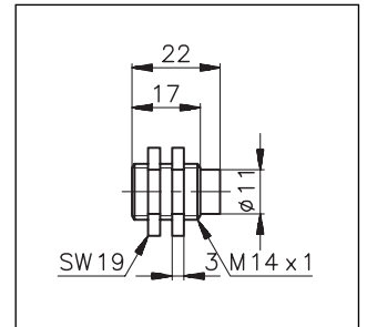
Dimensions (mm)
