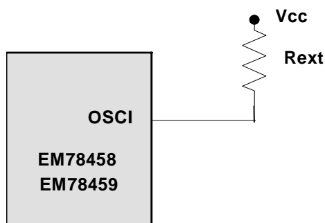
Fig. 23 Circuit for Internal C Oscillator Mode
