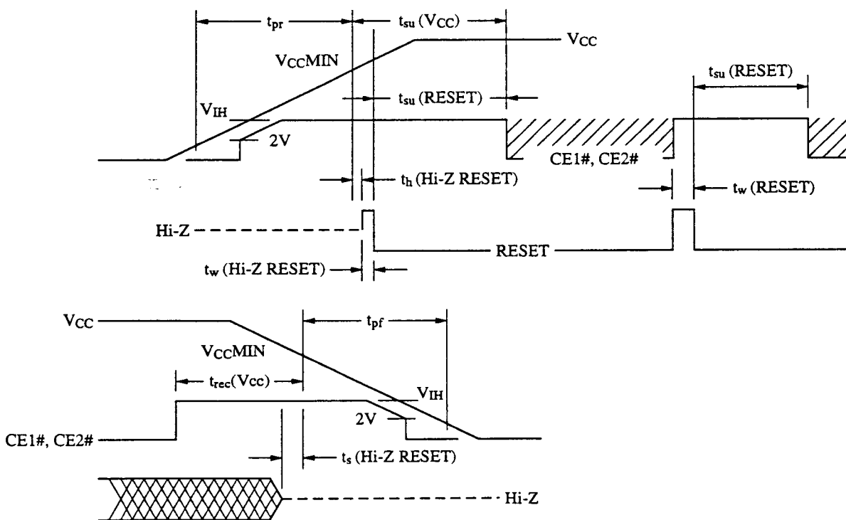
Power-Up/Down Timing for Systems Supporting RESET
