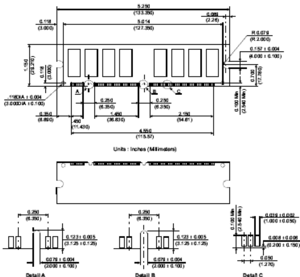
Figure 1: KVR133X64C3Q/128 168-Pin SDRAM Module
