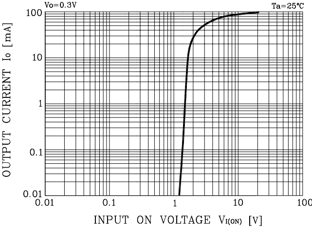
Fig. 1 I_o - V_{I(ON)}
