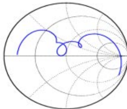
Output Smith Chart
