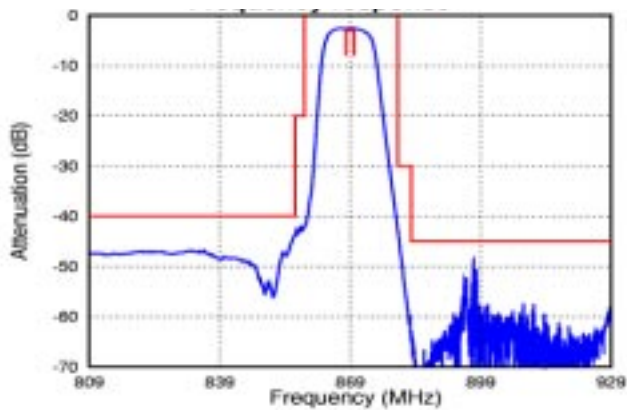
Frequency response
