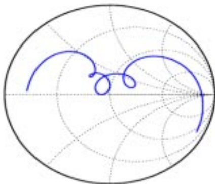
Input Smith Chart
