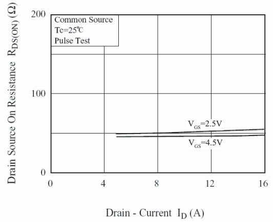
Fig2. R_{DS(on)} - I_D
