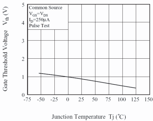
Fig5. V_{th} - T_j
