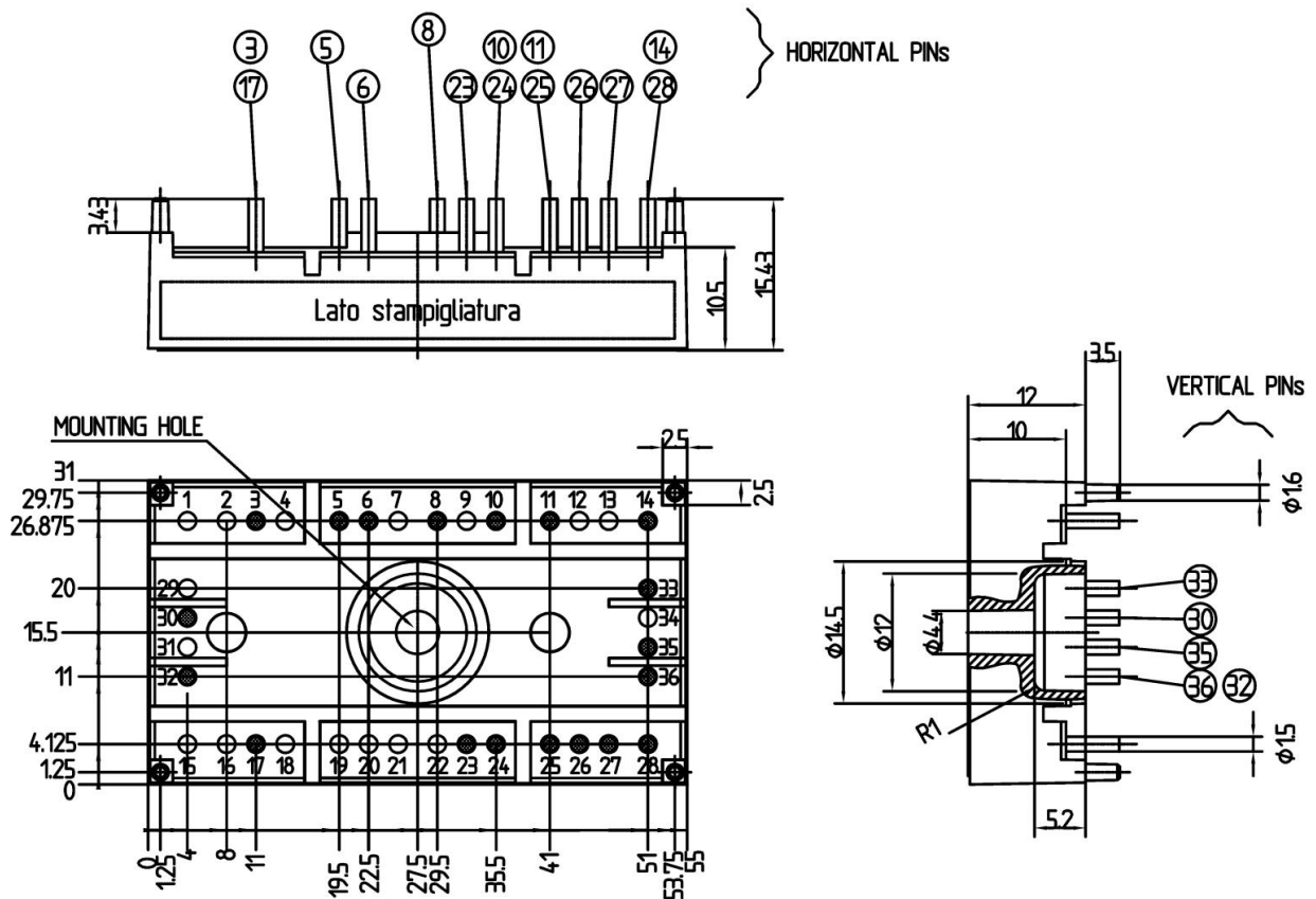
Case T 49 (Suggested hole diameter, in the PCB, for solder pins and plastic mounting pins: 2mm)
