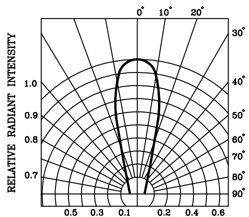
Fig.6 RADIATION DIAGRAM RADIATION DIAGRAM
