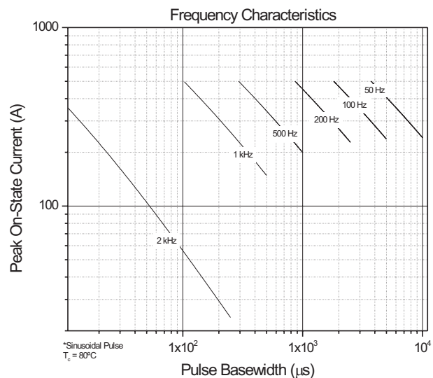
Fig. 9 - Frequency Characteristics
