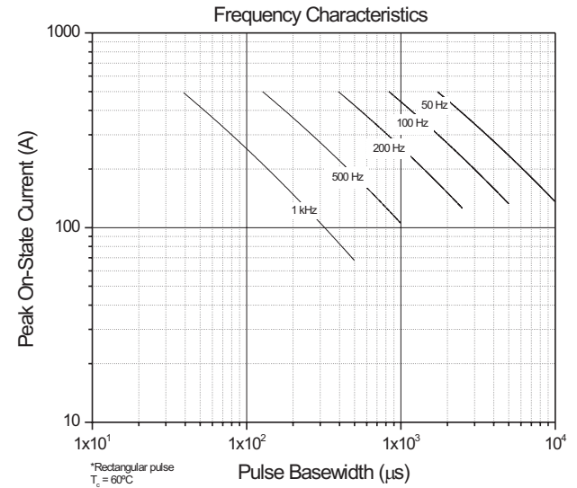
Fig. 8 - Frequency Characteristics
