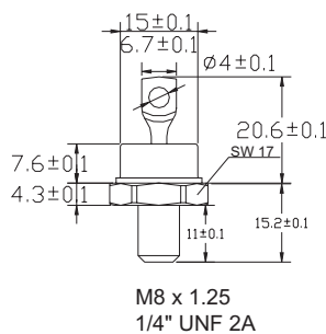
Fig. 15 - Outline Characteristics
