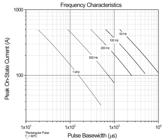
Fig. 10 - Frequency Characteristics
