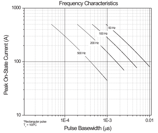
Fig. 12 - Frequency Characteristics
