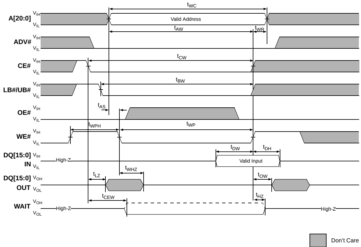
Figure 37. WE#-Controlled Asynchronous WRITE
