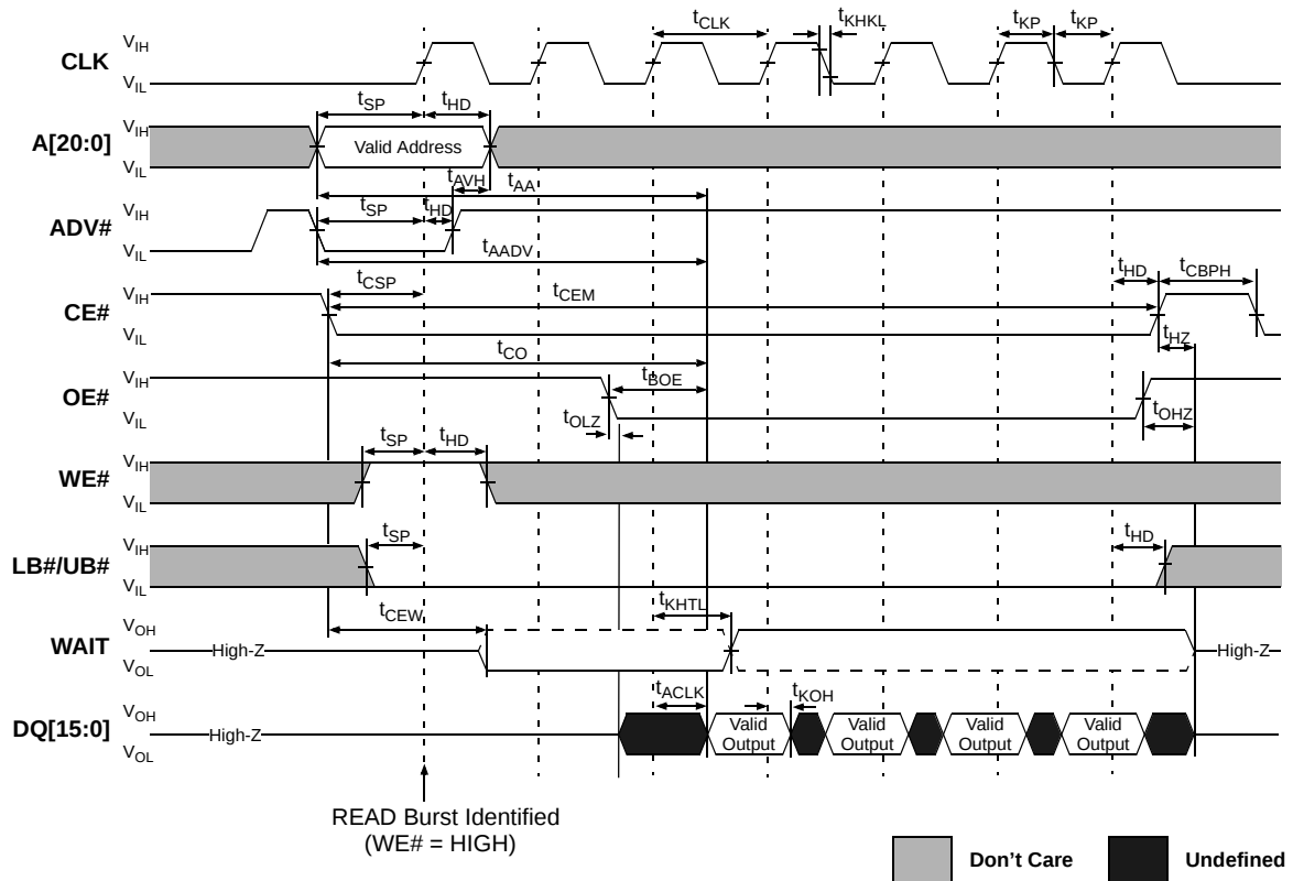
Figure 31. 4-Word Burst READ Operation - Fixed Latency
