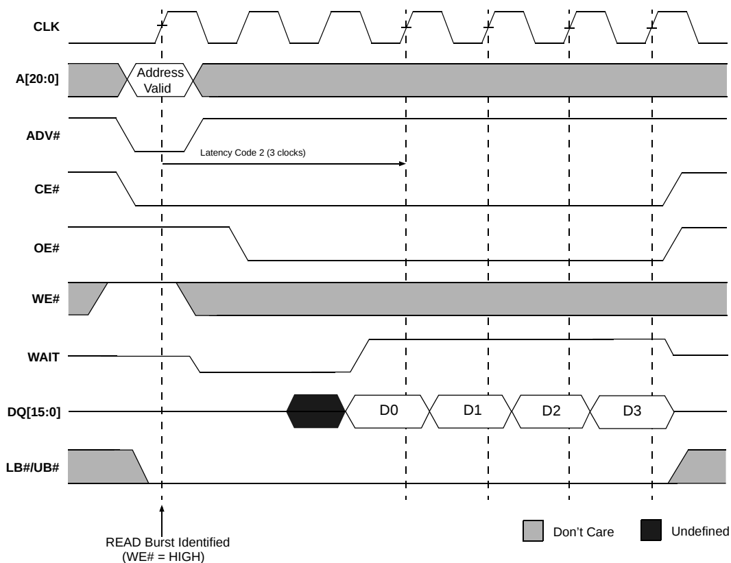
Figure 6: Burst Mode READ (4-word burst)
