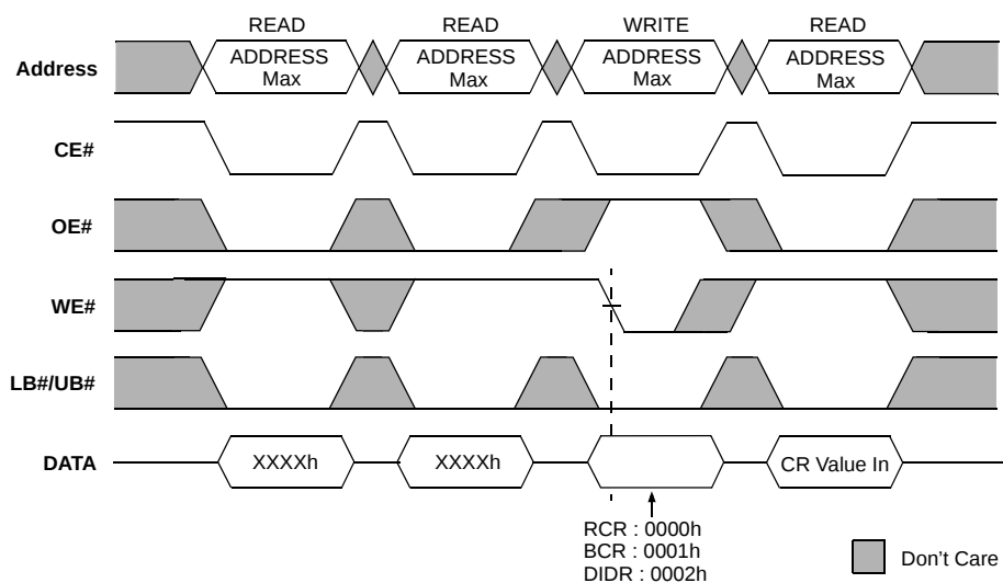
Figure 15: Read Configuration Register
