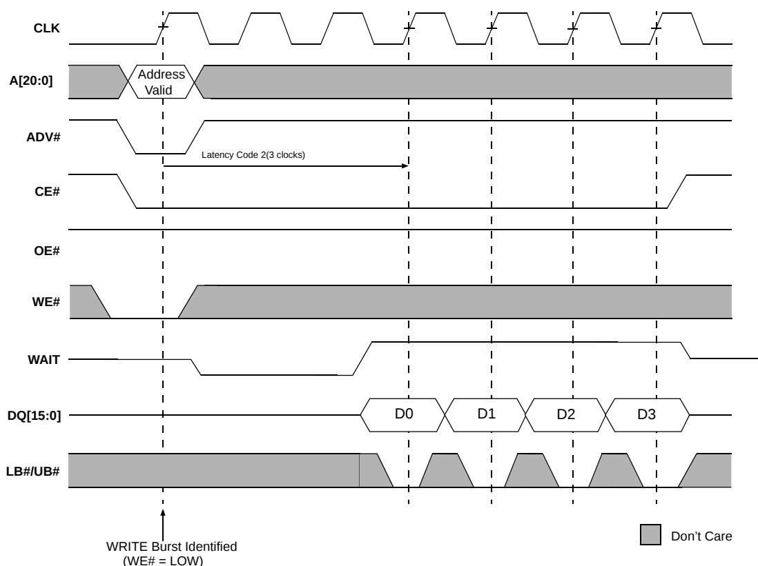
Figure 7: Burst Mode WRITE (4-word burst)
