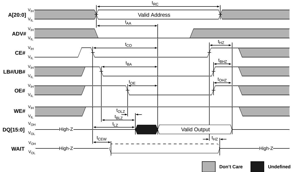
Figure 25: Asynchronous READ
