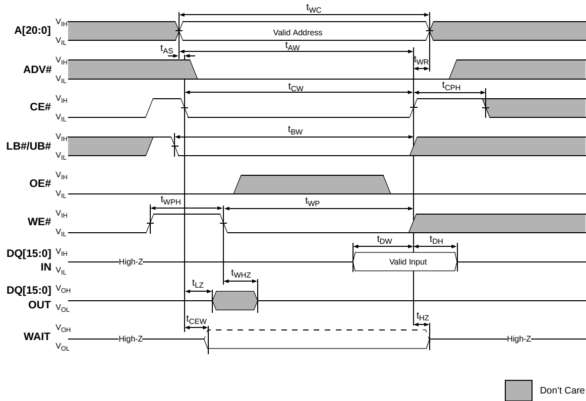
Figure 35. CE#-Controlled Asynchronous WRITE
