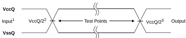
Figure 21: AC Input/Output Reference Waveform
