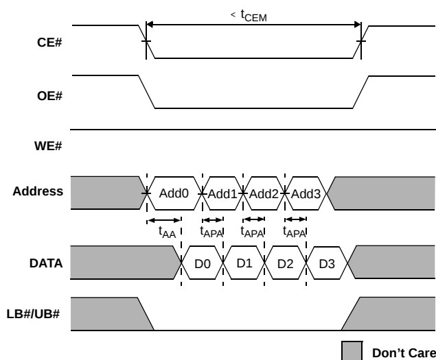
Figure 5: Page Mode READ Operation (ADV# LOW)
