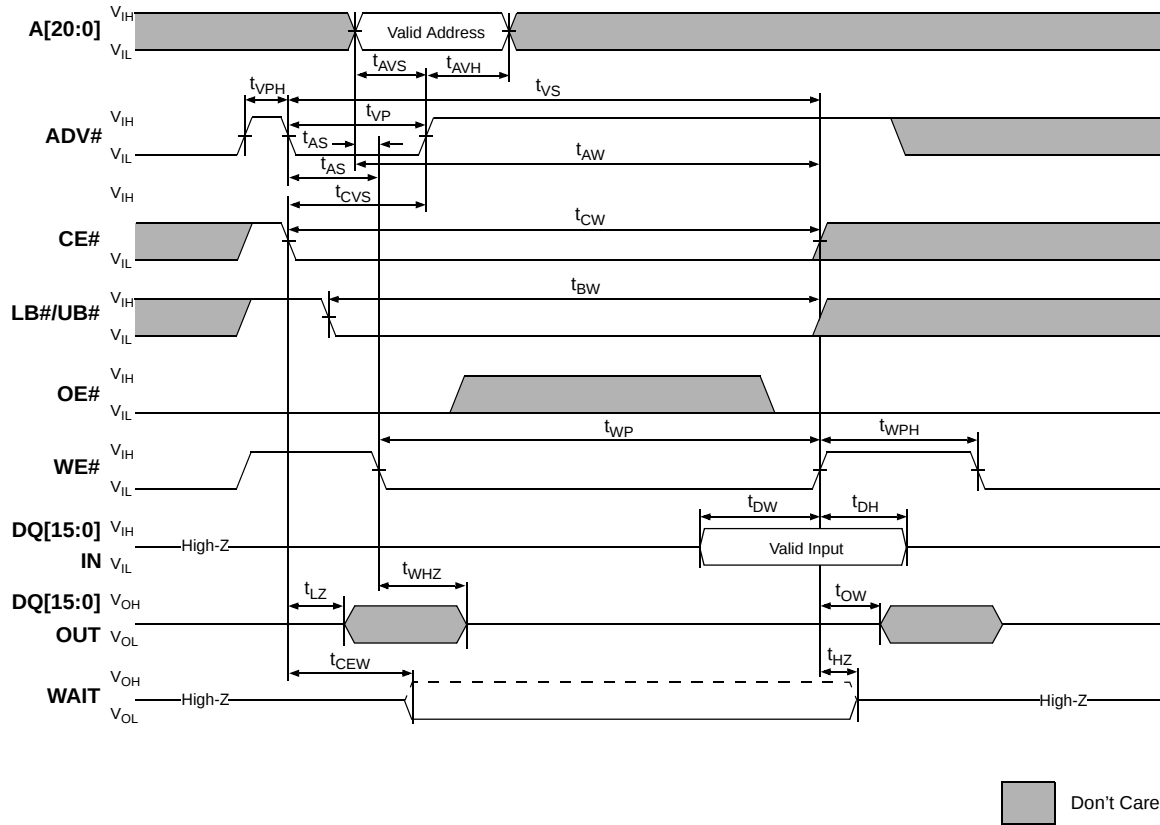
Figure 38. Asynchronous WRITE Using ADV#
