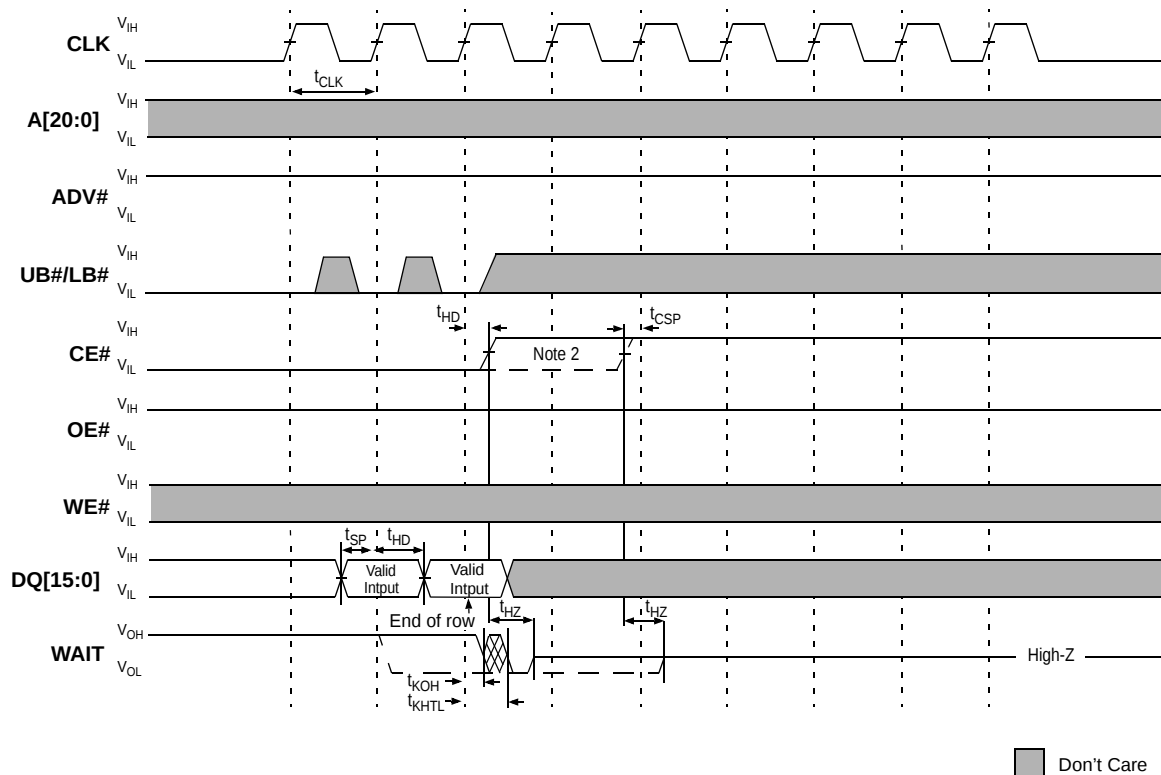
Figure 41. Burst WRITE at End-of-Row (Wrap Off)
