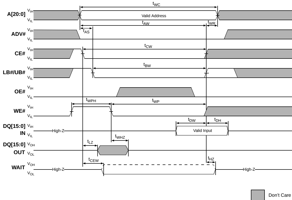
Figure 36. LB#/UB#-Controlled Asynchronous WRITE
