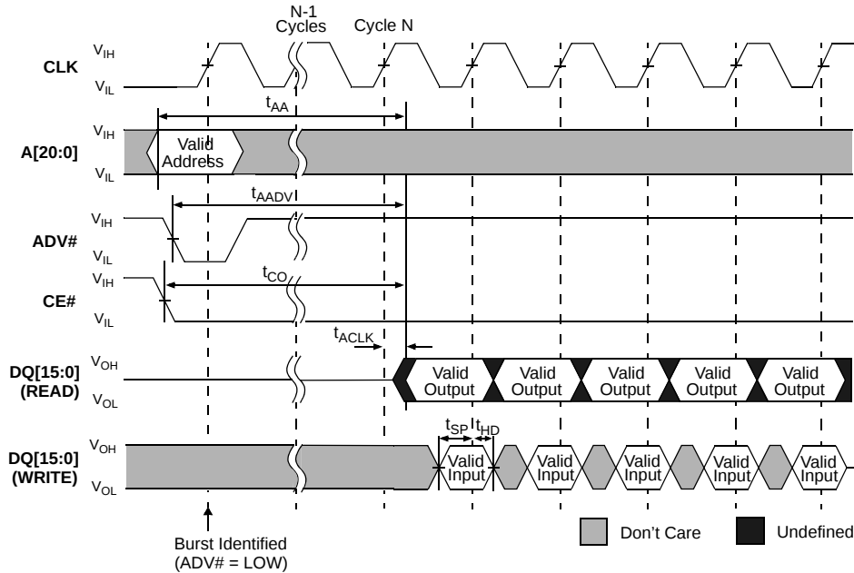
Figure 19: Latency Counter (Fixed Latency)
