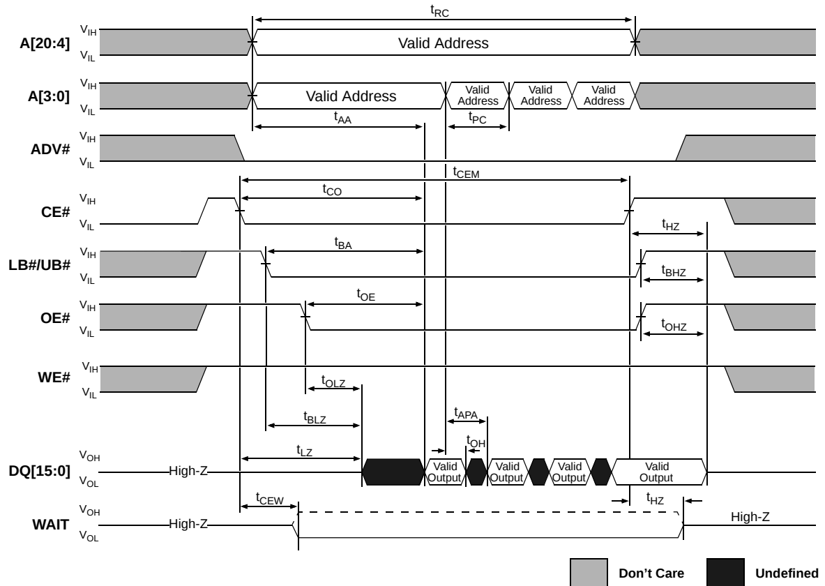
Figure 27: PAGE MODE READ
