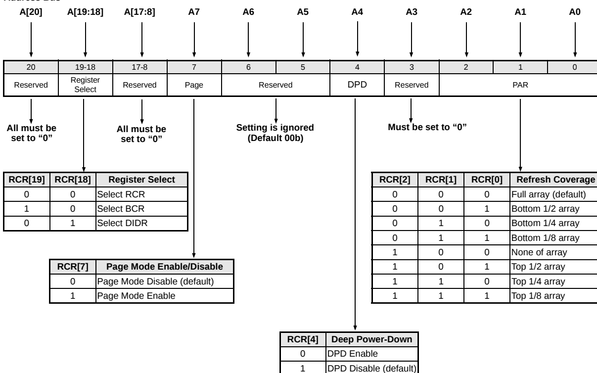
Figure 20: Refresh Configuration Register Mapping
