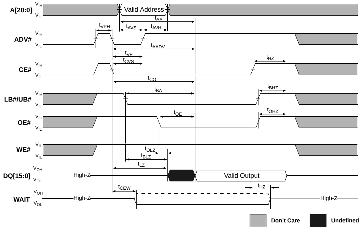
Figure 26: Asynchronous READ Using ADV#
