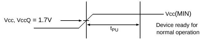
Figure 24: DPD Entry and Exit Timing Parameters
