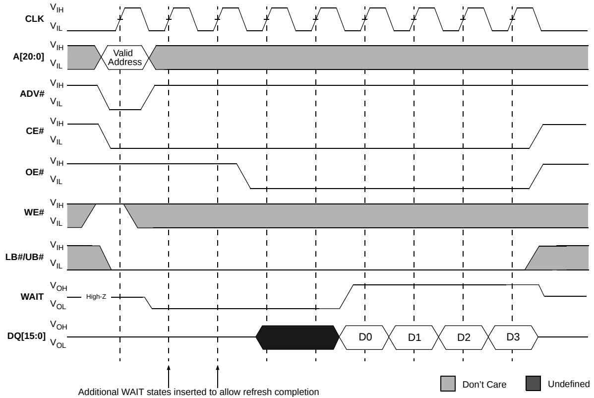
Figure 8: Refresh Collision During Variable-Latency READ Operation
