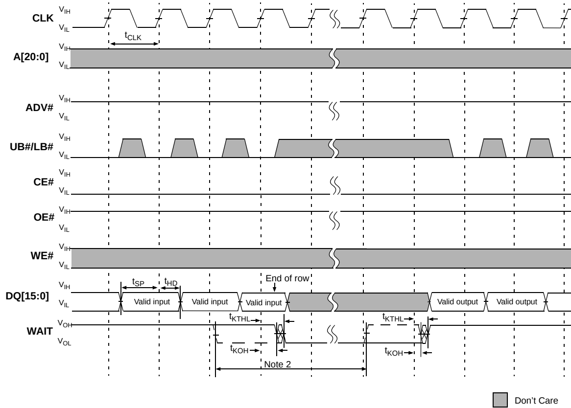
Figure 42. Burst WRITE Row boundary crossing
