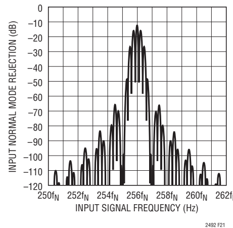
Figure 21. Input Normal Mode Rejection at f_S = 256 \cdot f_N
