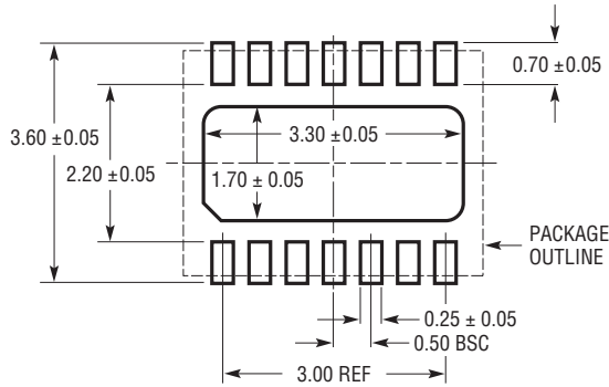
DE Package 14-Lead Plastic DFN (4mm × 3mm) (Reference LTC DWG # 05-08-1708 Rev A)
