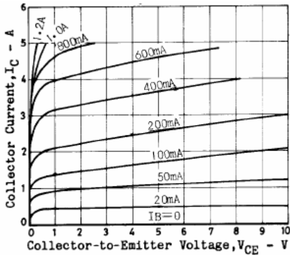
Fig.3 Static Characteristic
