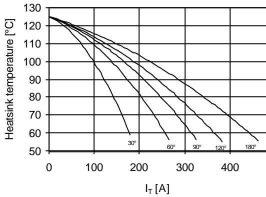
Current rating - sine wave
