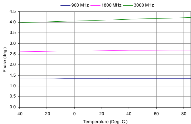
Figure 13. Relative Phase vs. Temperature: 7.75 dB State
