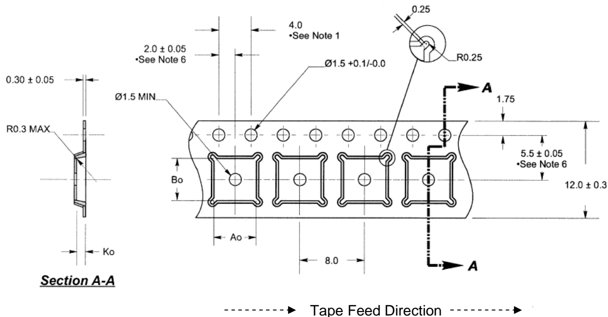
Figure 24. Tape and Reel Drawing
