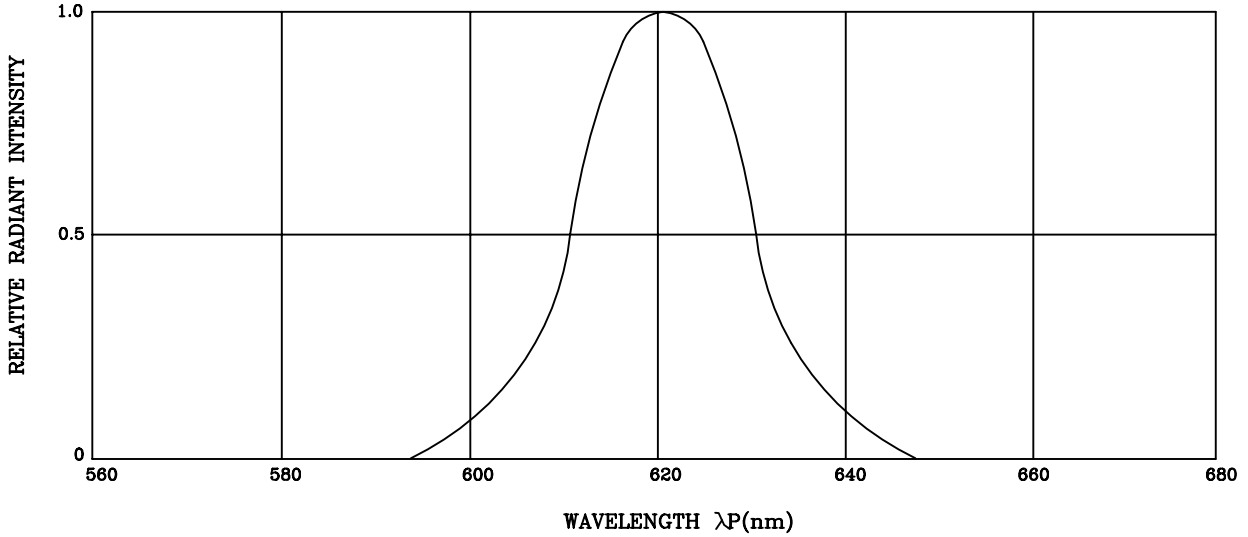
SPECTRAL DISTRIBUTION
